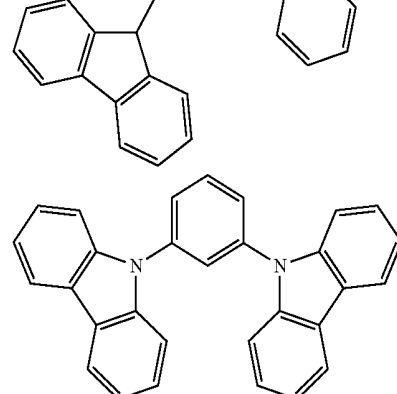
mCP
