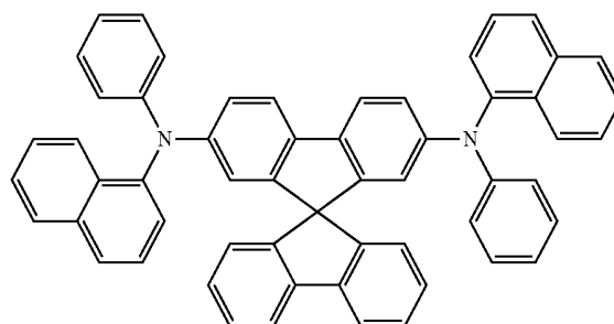
Spiro-NPB
