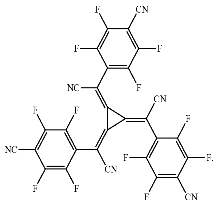
Compound HT-D2
